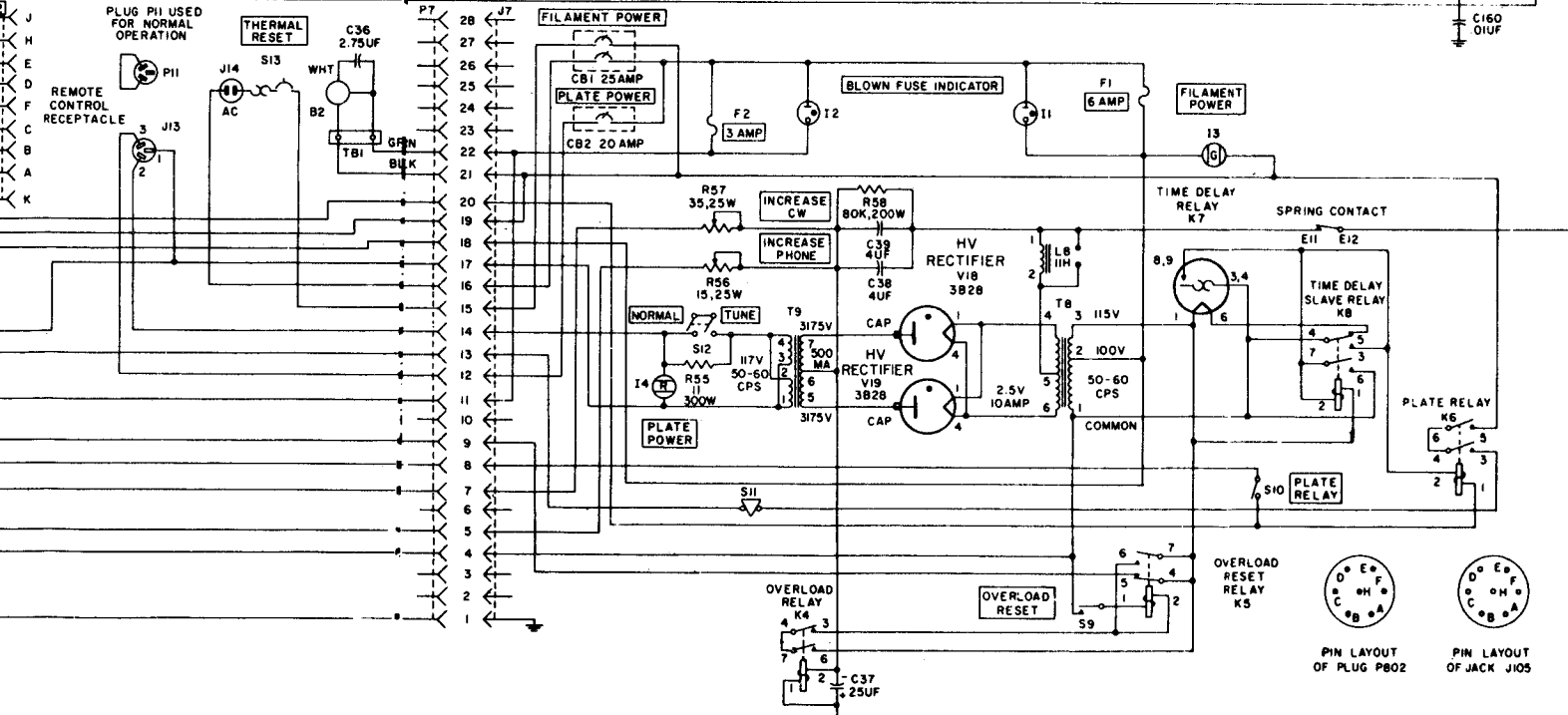
99. A model transmitter, complete schematic diagram.
